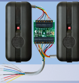
EXITRDR... Exit reader module for AxiomLite shown with two FR-360N readers
